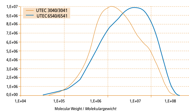
Figure 6 – UTEC Technology MWD curves. Abbildung 6 - UTEC Technologie, MWD-Kurven
