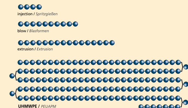
Figure 1 – Schematic drawing comparing polyethylenes for injection, blow and extrusion molding with UHMWPE polymeric chain.
